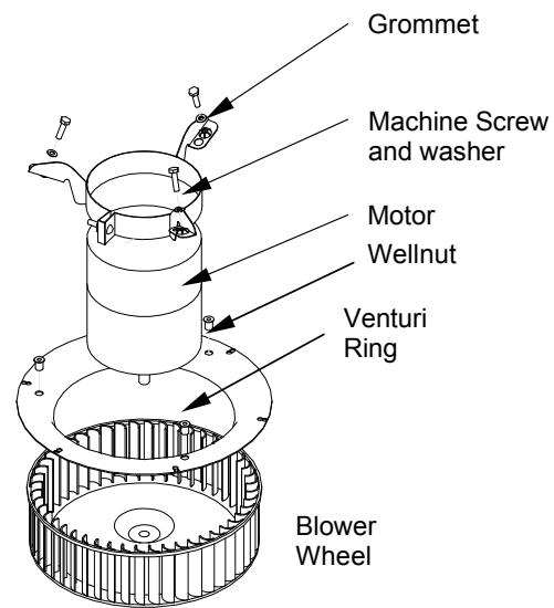
Motor Assembly
